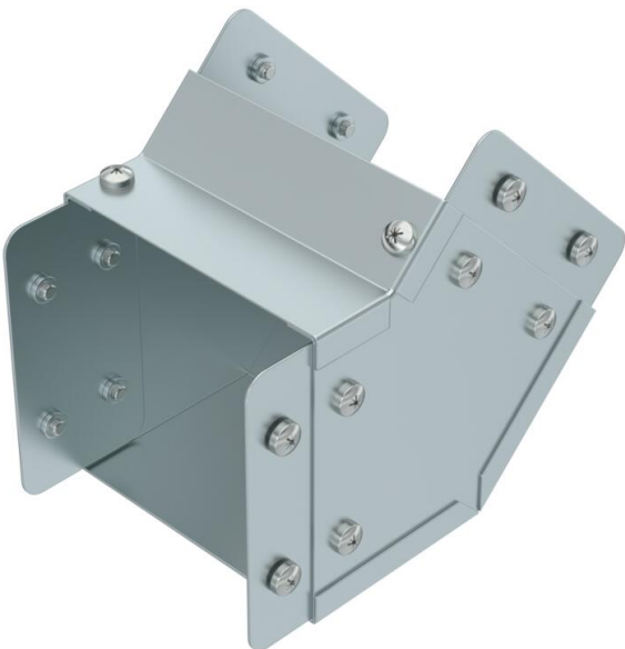
Single Compartment 45 Degree Internal Cover Bend, Pre-Galvanised Steel to suit Cable Trunking 100mm x 100mm
