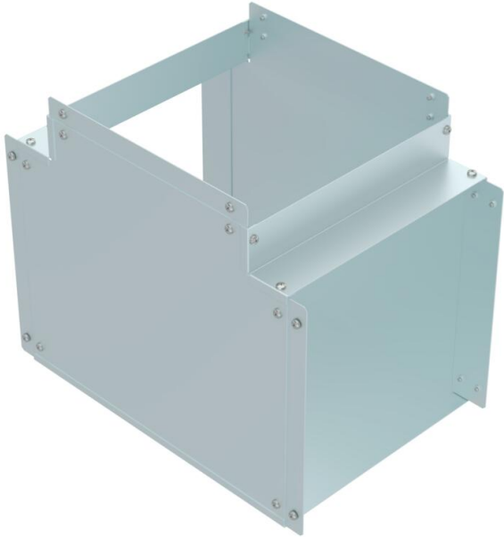
Single Compartment Tee Internal Cover, Non Gusset, Pre-Galvanised Steel to suit Cable Trunking 300mm x 300mm
