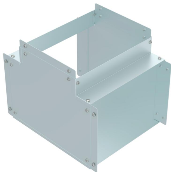
Single Compartment Tee Internal Cover, Non Gusset, Pre-Galvanised Steel to suit Cable Trunking 300mm x 225mm
